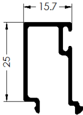
Ref. 1806 JUNQUILLO 25 mm
