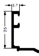
Ref. 1807 JUNQUILLO 25 mm
