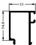
Ref. 1810 JUNQUILLO 25 mm
