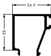
Ref. 9686 JUNQUILLO 25 mm
