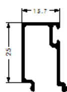
Ref. 1806 JUNQUILLO 25 mm
