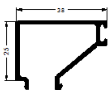
Ref. 15404 JUNQUILLO 25 mm
