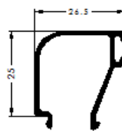
Ref. 9685 JUNQUILLO 25 mm
