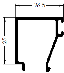
Ref. 9686 JUNQUILLO 25 mm
