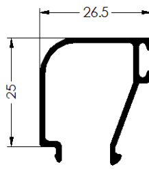
Ref. 9685 JUNQUILLO 25 mm
