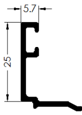
Ref. 1807 JUNQUILLO 25 mm
